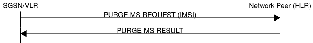
Figure 20: Purge MS (Normal Case)
