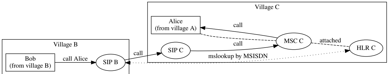
Figure 10: mslookup for connecting subscribers: Alice is visiting village C; a phone call gets routed directly to her current location independently from her resident village infrastructure
