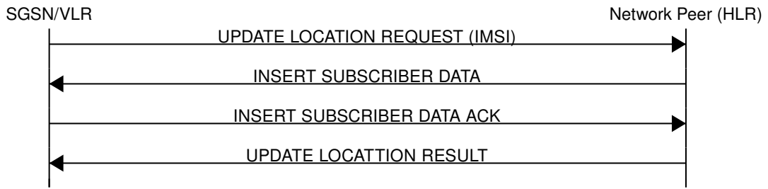
Figure 16: Update Location (Normal Case)
