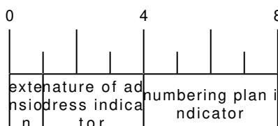
Figure 28: ToN/NPI header coding (as per 3GPP TS 129.002, MSB first)
