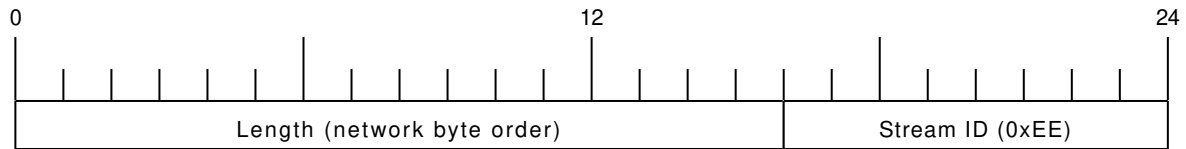
Figure 3: IPA header for control protocol
