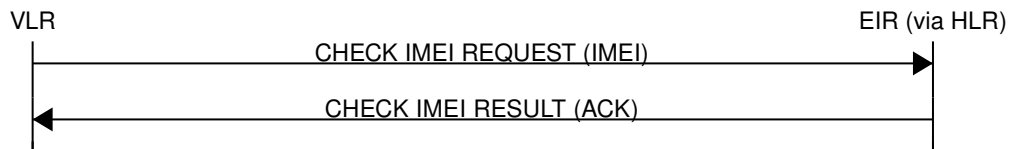
Figure 22: Check IMEI (Normal Case)
