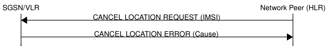
Figure 19: Cancel Location (Error Case)
