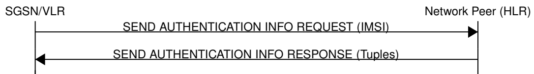
Figure 13: Send Authentication Info (Normal Case)
