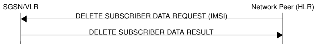
Figure 21: Delete Subscriber Data (Normal Case)
