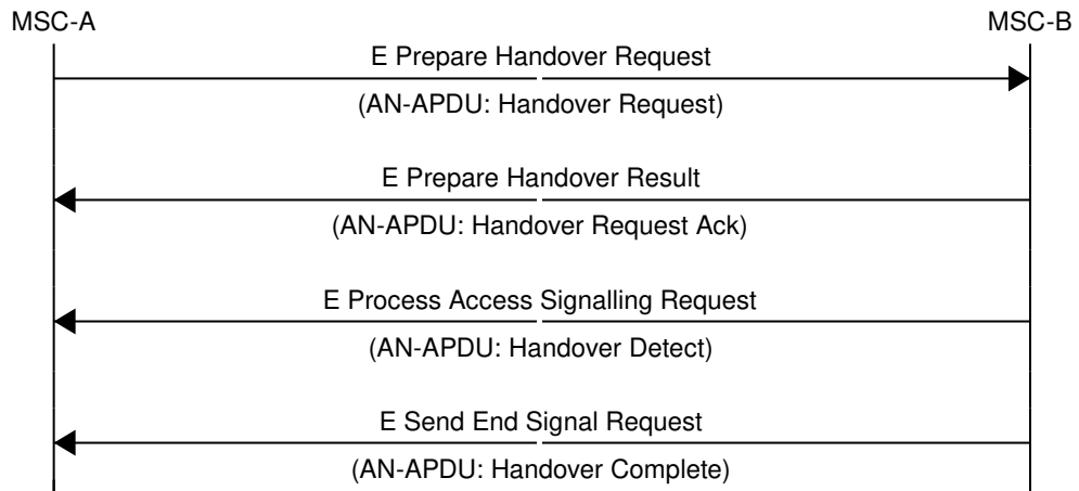
Figure 23: E Handover (Normal Case)
