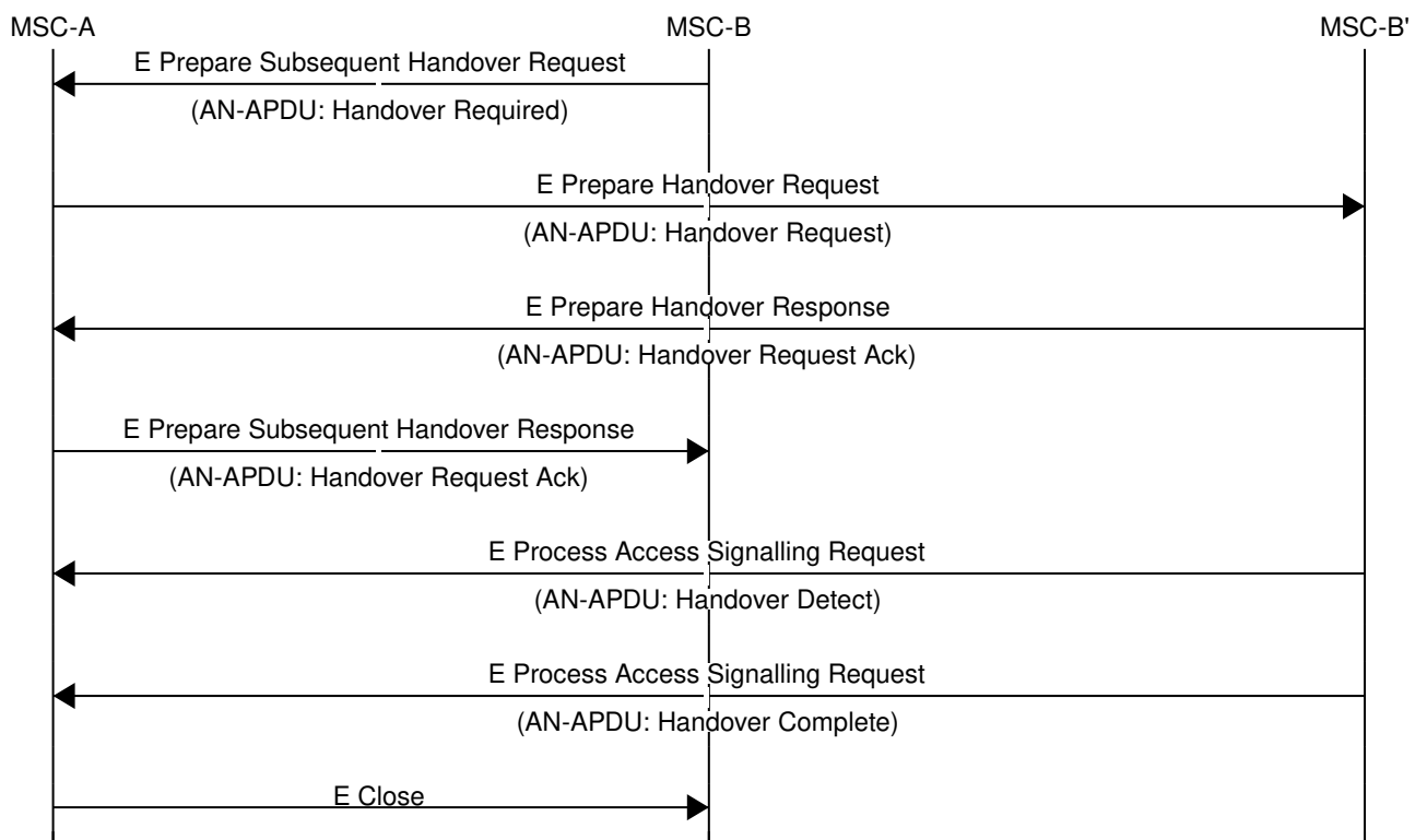
Figure 24: E Subsequent Handover (Normal Case)
