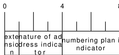
Figure 28: ToN/NPI header coding (as per 3GPP TS 129.002, MSB first)
