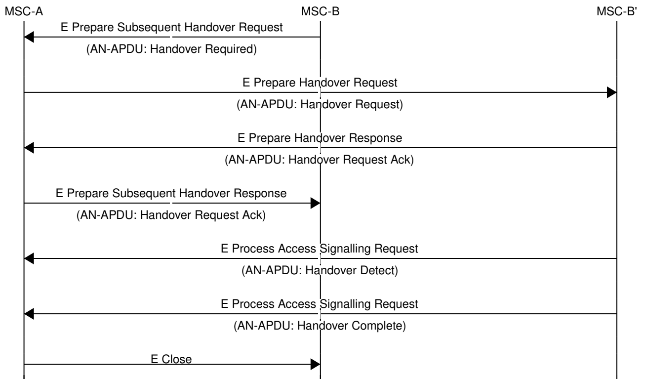
Figure 21: E Subsequent Handover (Normal Case)
