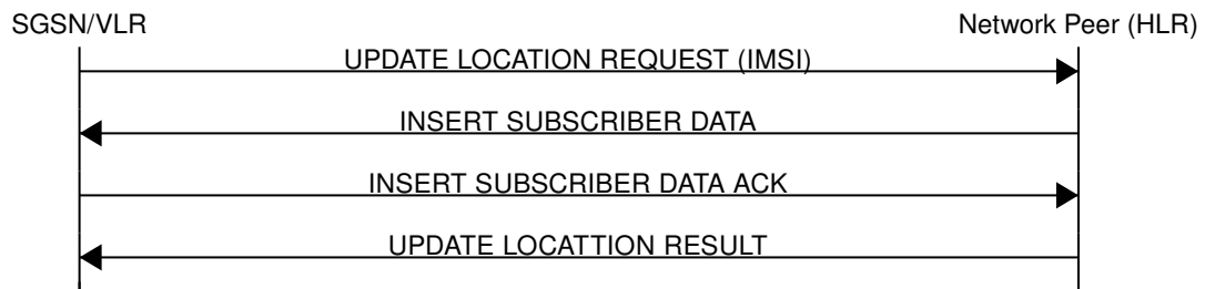
Figure 13: Update Location (Normal Case)
