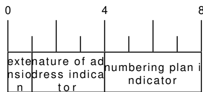
Figure 25: ToN/NPI header coding (as per 3GPP TS 129.002, MSB first)
