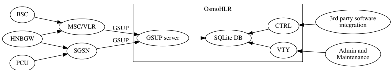
Figure 1: Typical GSM network architecture used with OsmoHLR
