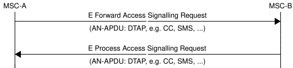
Figure 22: E Process and Forward Access Signalling (Normal Case)
