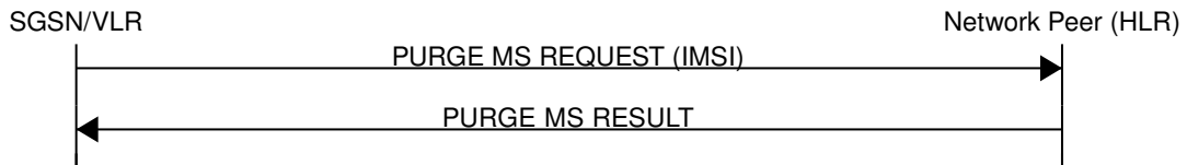
Figure 17: Purge MS (Normal Case)
