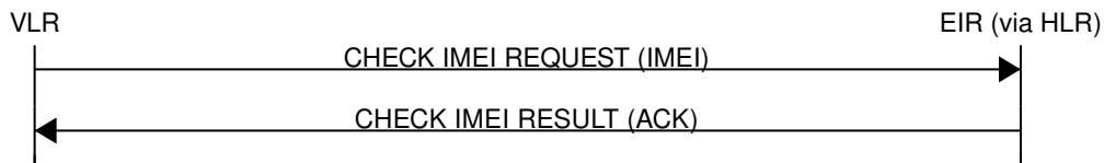
Figure 19: Check IMEI (Normal Case)
