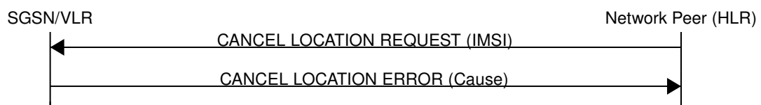
Figure 16: Cancel Location (Error Case)
