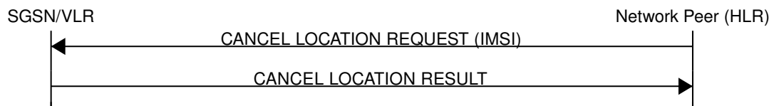
Figure 15: Cancel Location (Normal Case)
