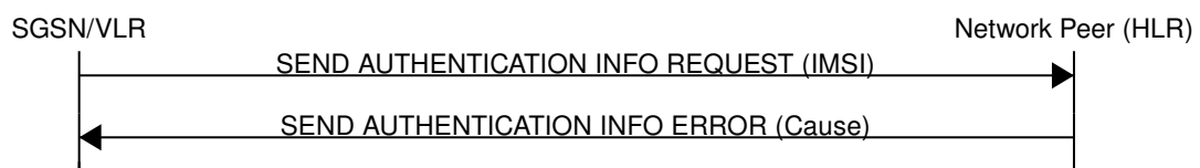
Figure 11: Send Authentication Info (Erroneous Case)
