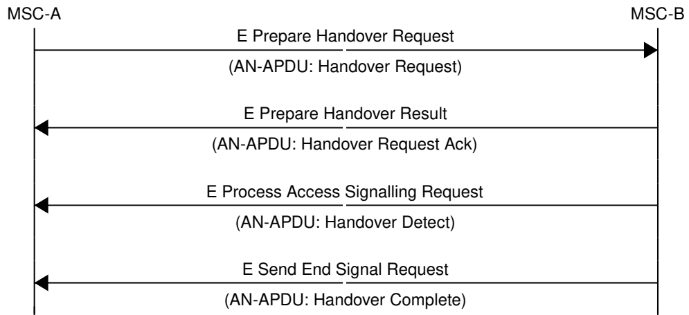
Figure 20: E Handover (Normal Case)
