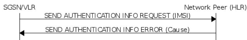
Figure 14: Send Authentication Info (Erroneous Case)
